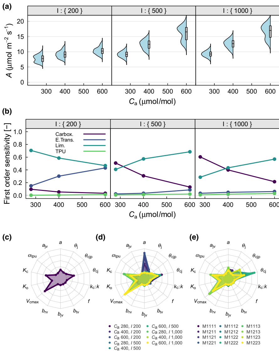
FIGURE 3 Sensitivity of carbon assimilation ( A , \mu\text{mol m}^{-2} \text{s}^{-1} ) to variability in processes and parameters across various C_a and I environmental conditions. (a) Semi-violin plots showing distributions of A against C_a ( \mu\text{mol/mol} , x-axis) and I ( \mu\text{mol m}^{-2} \text{s}^{-1} , panels) boxes represent the interquartile range and median, whiskers the full range. (b) First order sensitivity index of A to variability in the four processes against C_a ( \mu\text{mol/mol} , x-axis) and I ( \mu\text{mol m}^{-2} \text{s}^{-1} , panels). (c) First order sensitivity index of A to variability in the 14 parameters, indexes integrated across the 12 models and nine environmental conditions. (d) First order sensitivity index of A to variability in the 14 parameters, indexes integrated across the 12 models and colour coded for each of the nine environmental conditions. (e) First order sensitivity index of A to variability in the 14 parameters, indexes integrated across the nine environmental conditions and colour coded for each of the 12 models
