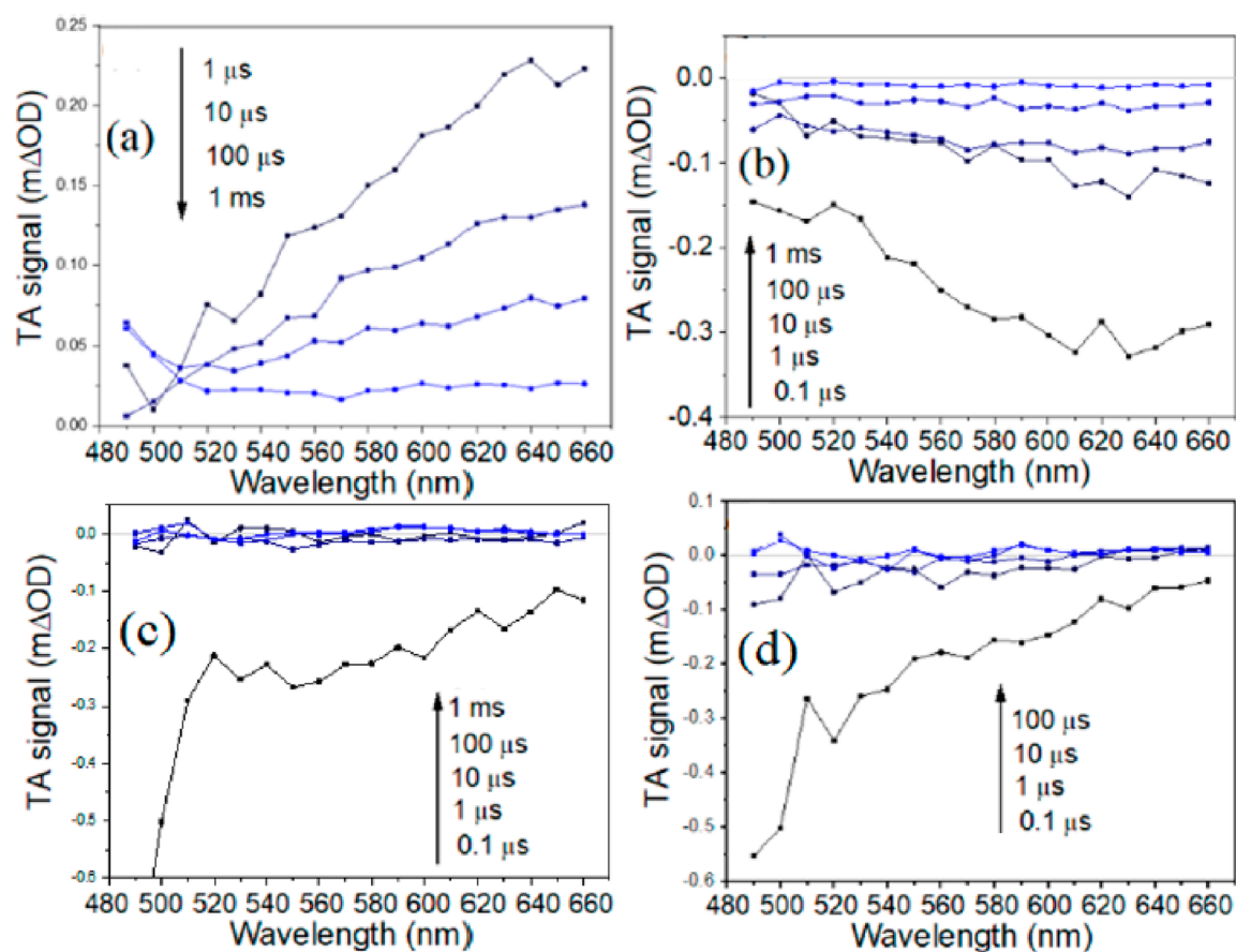
Figure 4. TAS spectra obtained in N 2 atmosphere after 355 nm excitation (200 Hz, 850 μJ/cm 2 /pulse) of (a) ref-g-C 3 N 4 sample, (b) def-g-C 3 N 4 -1 sample, (c) def-g-C 3 N 4 -2 sample, and (d) def-g-C 3 N 4 -5 sample.
