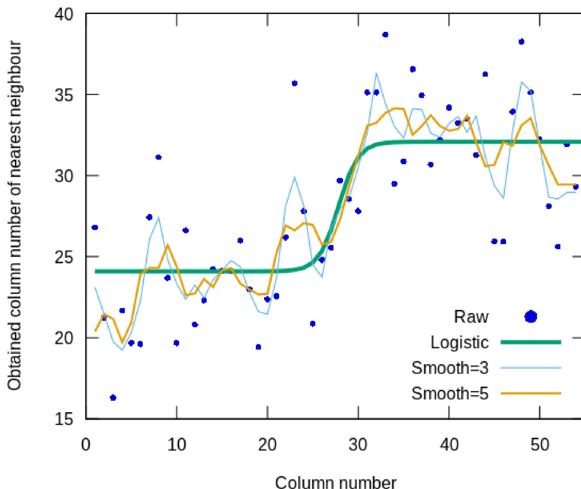
Fig 10. Average serial column position of the nearest-neighbour of a column, measured in fraglet-feature space. Raw samples (points), curves smoothed over 3 and over 5 points, and a best-fit logistic curve.
