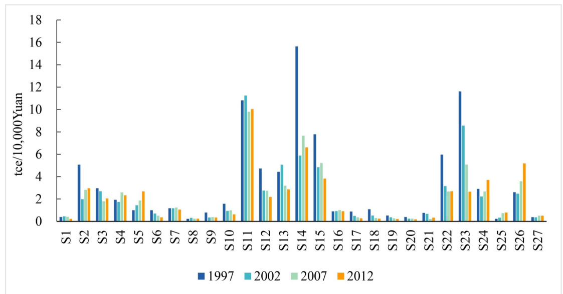
Fig 1. Comparison of Chinese sectoral energy intensities in 1997, 2002, 2007, and 2012.
